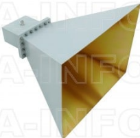
LB-975-15-C-7/16F Standard Gain Horn Antenna 0.75-1.12GHz 15dB Gain 7/16(DIN) Female
